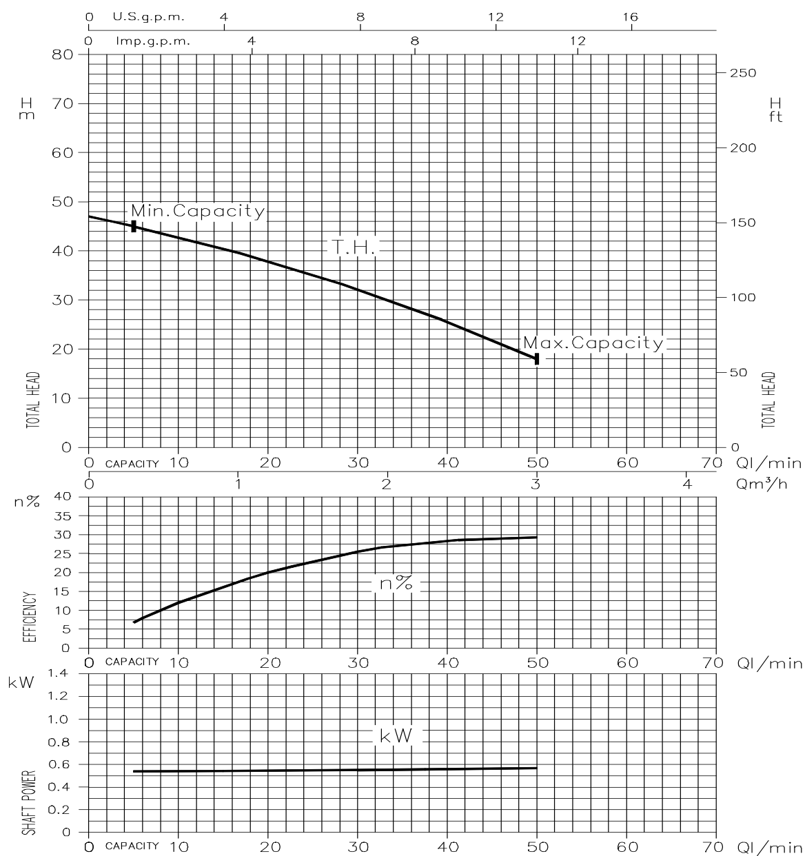
AGA 0.75 - Impeller diameter = 130 mm
