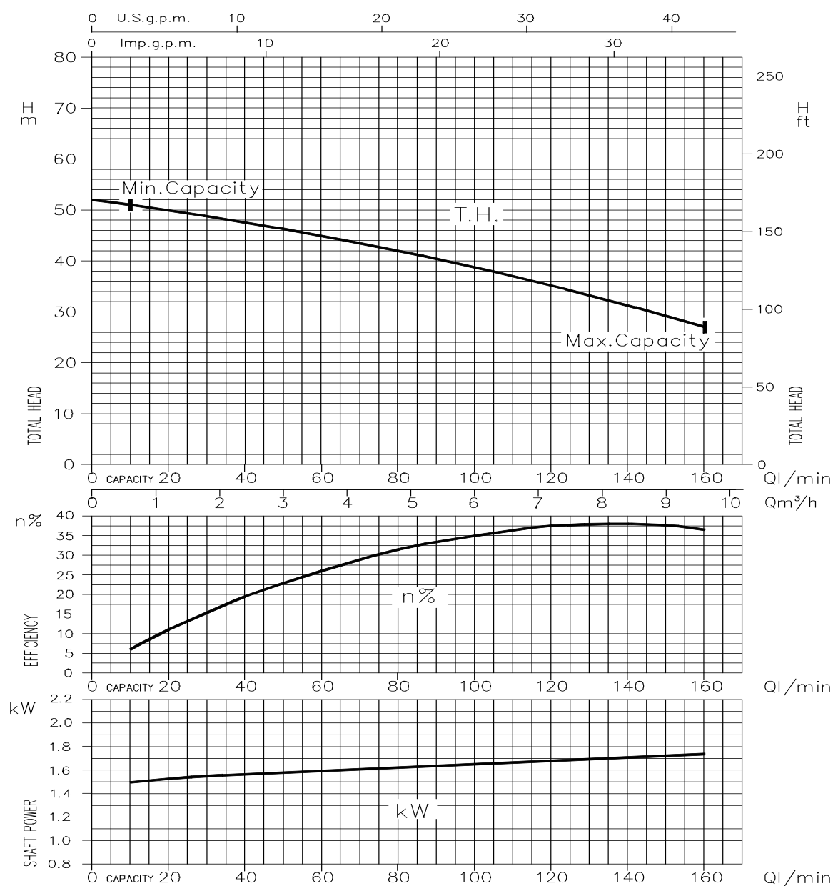
AGC 2.00 - Impeller diameter = 157 mm
