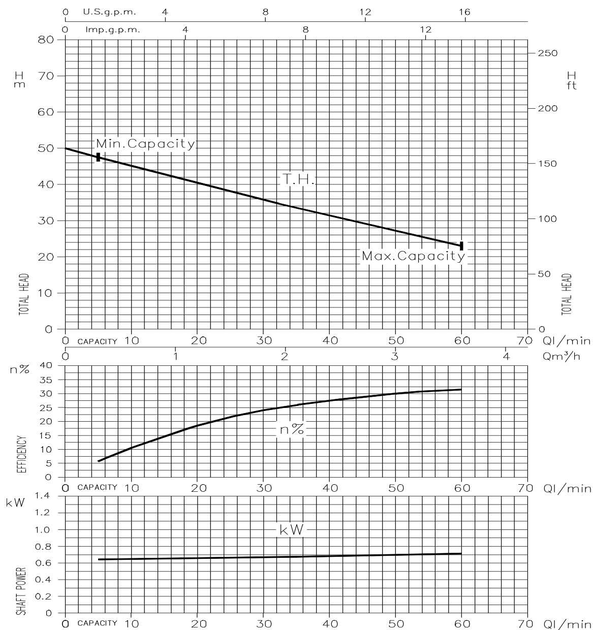
AGA 1.00 - Impeller diameter = 130 mm
