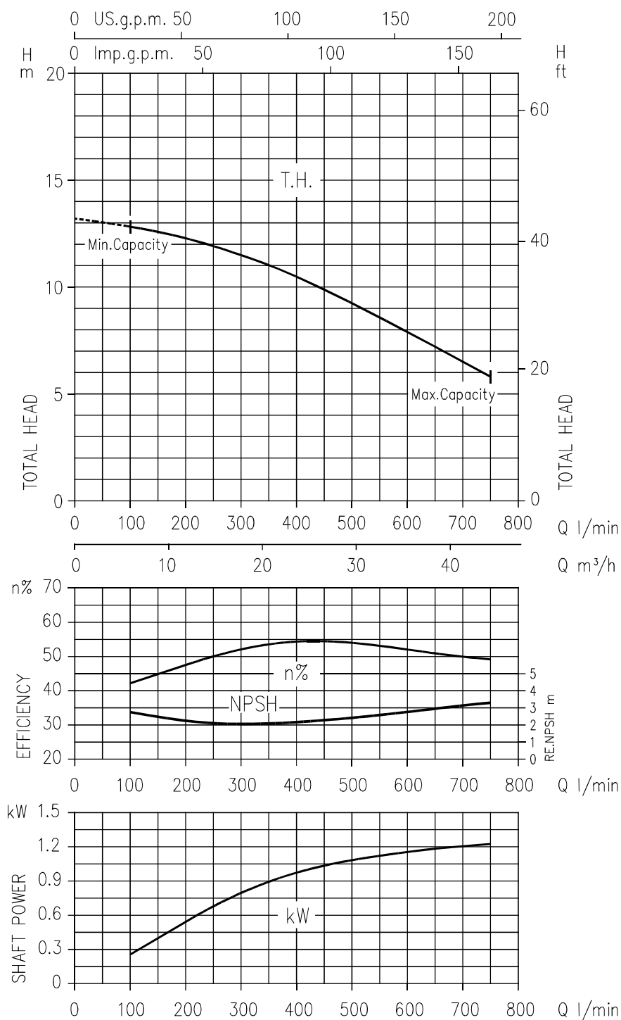
DWO 200 - Impeller diameter = 103 mm
